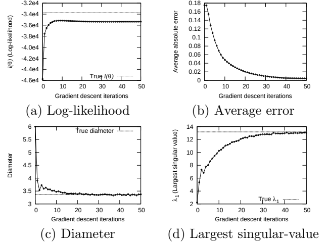
Figure 2. Convergence of graph patterns with the number of iterations of gradient descent using synthetic dataset.
