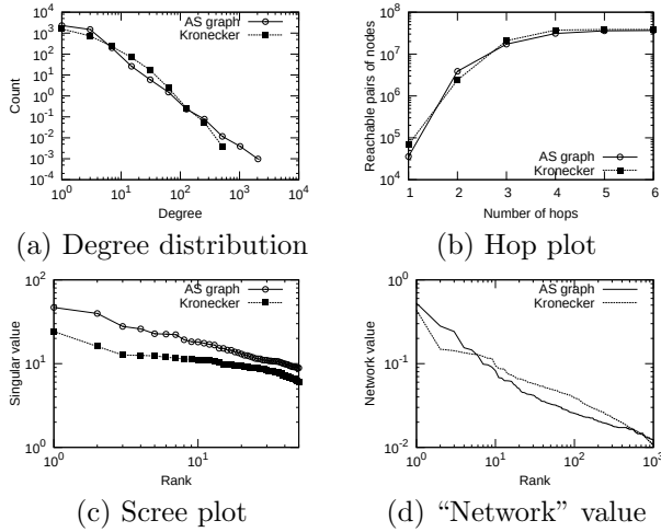
Figure 3. Autonomous Systems : Overlaid patterns of real graph and the fitted Kronecker graph. Notice that the fitted Kronecker graph matches patterns of the real graph.
