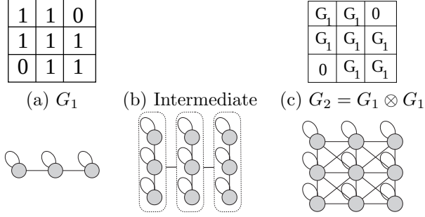
Figure 1. Kronecker multiplication : Top row: structure of adjacency matrices. Bottom: corresponding graphs – “3-chain” and its Kronecker product with itself; each of the nodes gets expanded into 3 nodes, which are then linked.
