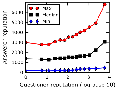
Figure 3: Max/median/min answerer reputation as a function of the questioner reputation.
