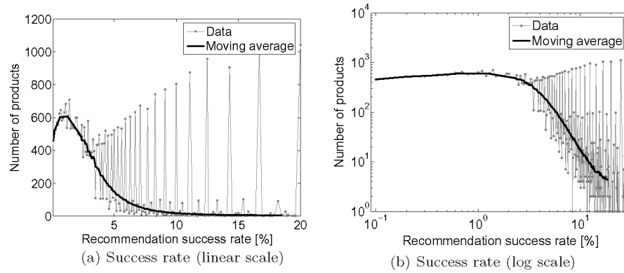
Fig. 16. Distribution of product recommendation success rates. Both plots show the same data: (a) on a linear (lin-lin) scale, and (b) on a logarithmic (log-log) scale. The bold line presents the moving average smoothing.
