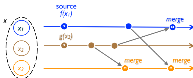
Figure 4: State-based replication
