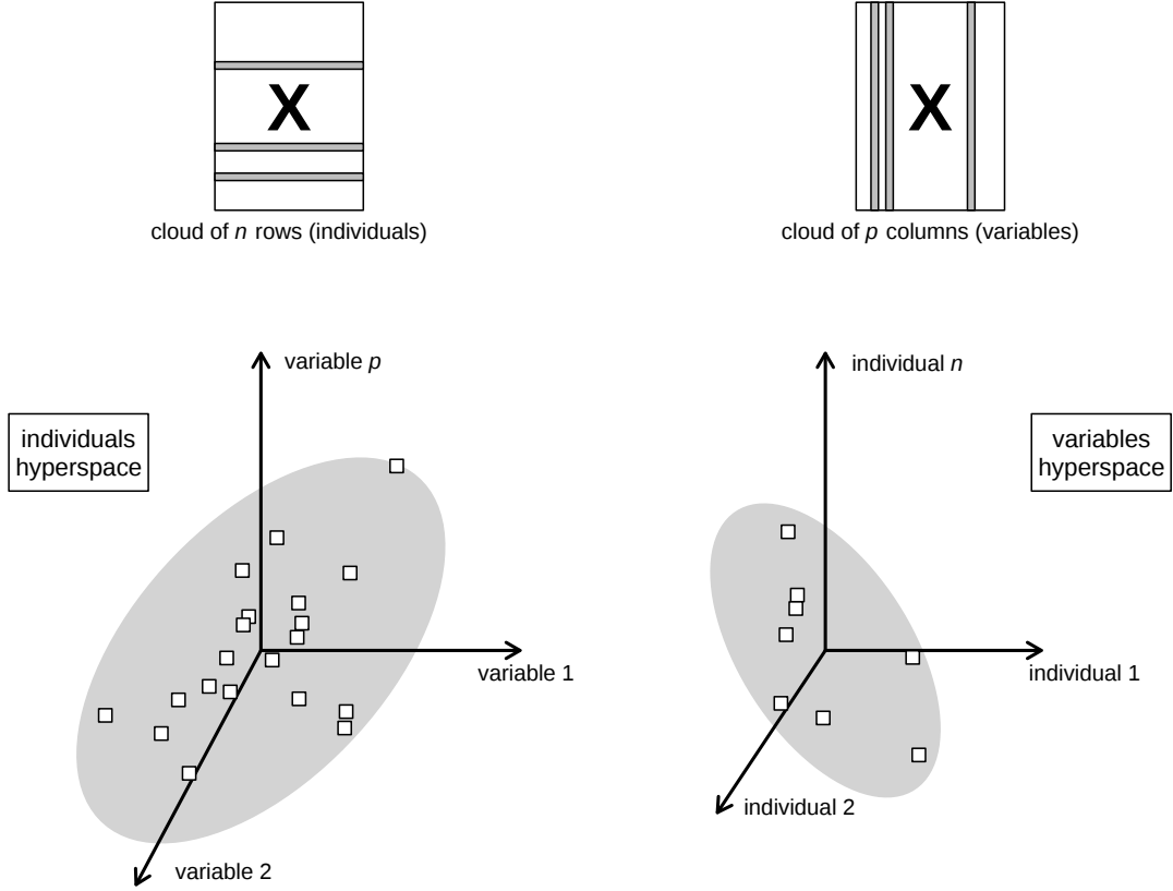
Figure 1: Representation of table \mathbf{X} as a cloud of n points (individuals) in an hyperspace with p dimensions (variables) or as a cloud of p points (variables) in an hyperspace with n dimensions (individuals)
