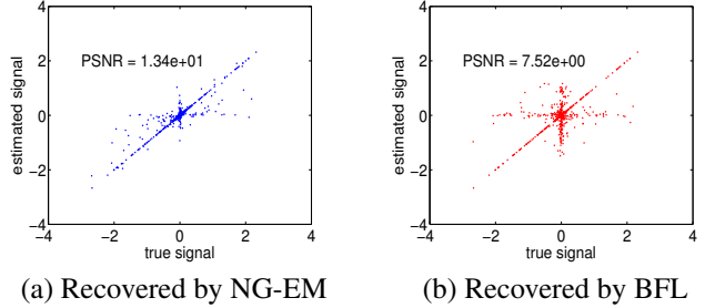
Figure 1. Recovery of the causal-frequency data using the proposed EM method and the traditional methods: (a) The recovery results of the proposed NG-EM method ( PSNR = 13.4 ); (b) The recovery results of the BFL method ( PSNR = 7.52 ).
