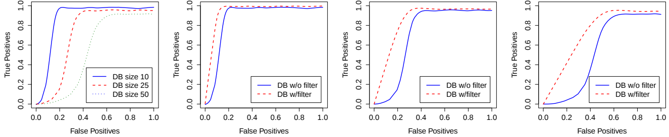
(a) ROC curves for all (b) Database size 10 (c) Database size 25 (d) Database size 50 Figure 7: Comparing ROC curves for different database sizes in (a), and comparing ROC curves with and without filtering entries based on inter K-S scores in (b)-(d).
