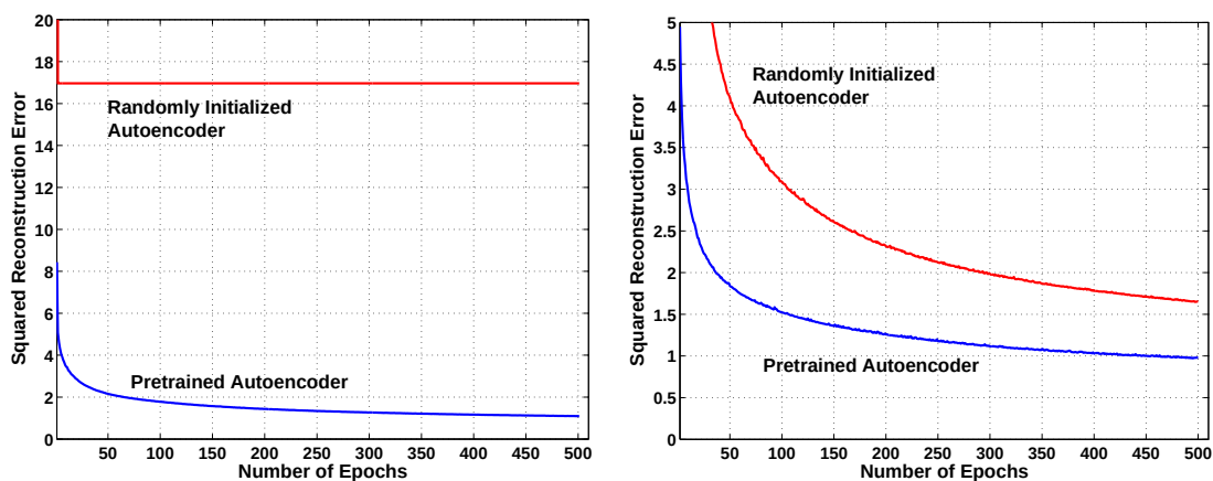
Fig. S1: The average squared reconstruction error per test image during fine-tuning on the curves training data. Left panel: The deep 784-400-200-100-50-25-6 autoencoder makes rapid progress after pretraining but no progress without pretraining. Right panel: A shallow 784-532-6 autoencoder can learn without pretraining but pretraining makes the fine-tuning much faster, and the pretraining takes less time than 10 iterations of fine-tuning.
