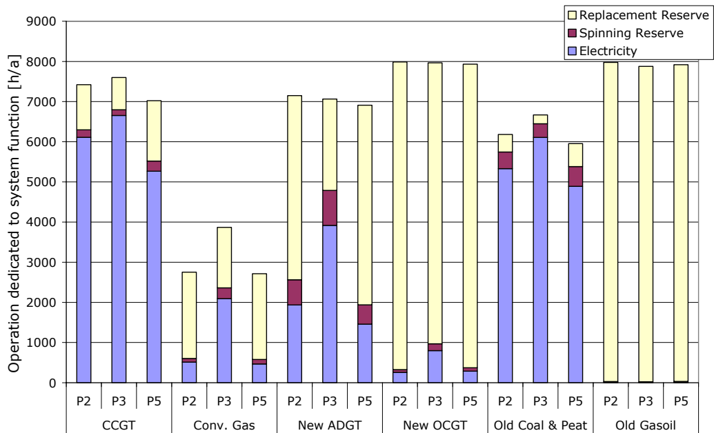
Figure 3-9: Operational modes of conventional generation portfolios 2, 3 and 5
