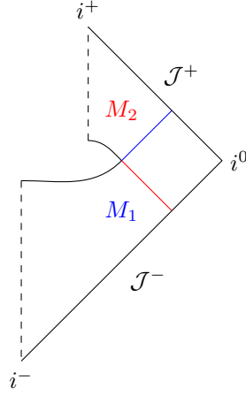
Figure 4.8: Penrose diagram of a fully evaporating black hole with a removed high curvature region
