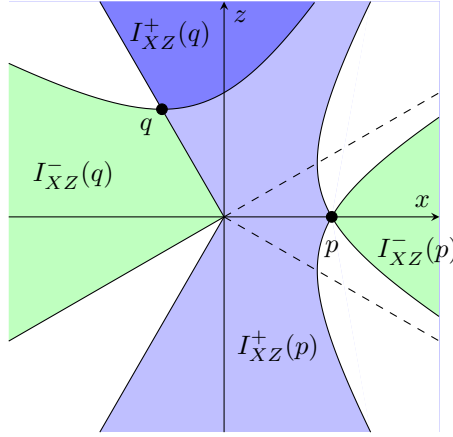
Figure 5.3: The points p, q of Example 5.17 and their futures and pasts (restricted to the (x, z) -plane XZ ).
