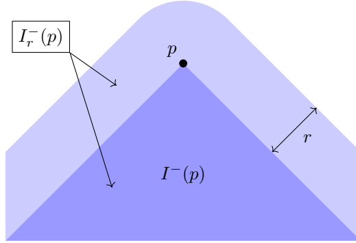
Figure 4.2: The sets I^-(p) (dark blue) and I_r^-(p) (light and dark blue) for some point p in Minkowski spacetime, with d the Euclidean distance.
