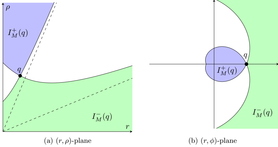
Figure 5.4: The causal structure of an isotropic neighborhood.
