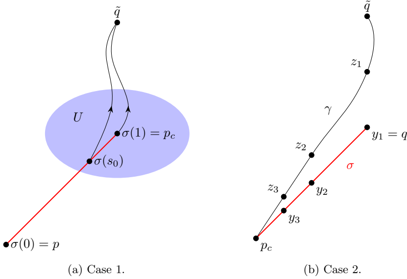
Figure 5.1: An illustration of the proof of Lemma 5.12. The red line represents \sigma , and the black curves represent future-directed causal curves.
