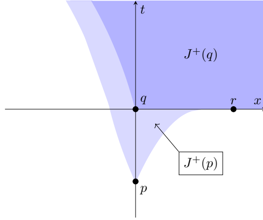
Figure 2.2: The points p, q, r in Example 2.17, which satisfy (p, q) \in \text{Int } J^+ and (q, r) \in J^+ but (p, r) \notin \text{Int } J^+ .
