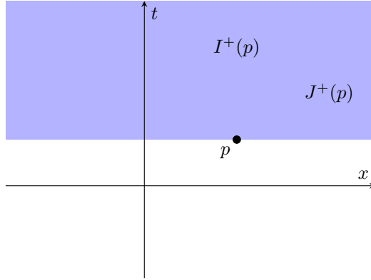
Figure 4.1: The sets I^+(p) (blue, without boundary) and J^+(p) = I^+(p) \cup \{p\} for a point p in Example 4.35.
