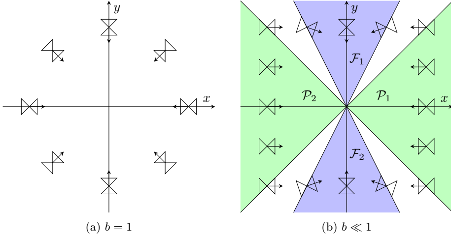
Figure 5.2: The causal structure of Example 5.16.
