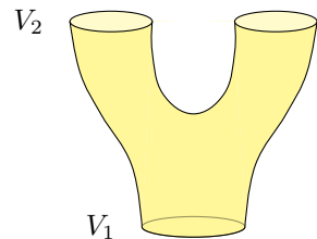
Figure 1.3: A cobordism.
