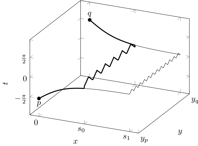
Figure 6.3: Two piecewise causal curves going through the points p_{s_0} and q_{s_0} (thick) and p_{s_1} and q_{s_1} (thin), respectively, that approximate the null distance between p and q in Example 6.33. The thin curve yields a better approximation.
