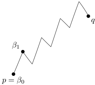
Figure 1.8: A piecewise causal curve \beta from p to q , with alternating future- and past-directed pieces.
