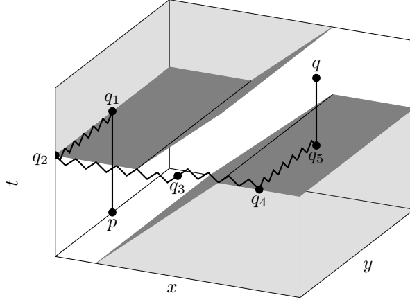
Figure 6.4: A piecewise causal curve that approximates the null distance between p and q in Example 6.34. Only the space in between the two grey surfaces is part of the spacetime. The curve comes \varepsilon -close to the boundary, but remains entirely within M .
