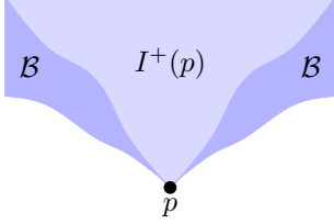
Figure 1.7: A causal bubble \mathcal{B} . Here J^+(p) = I^+(p) \cup \mathcal{B} .
