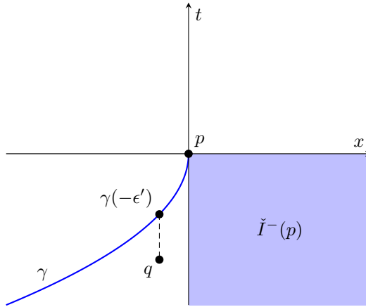
Figure 2.1: The spacetime of Example 2.8, with the curve \gamma that lies outside of \check{I}^-(p) , while nonetheless (\gamma(-\epsilon'), p) \in \check{I}^+ .
