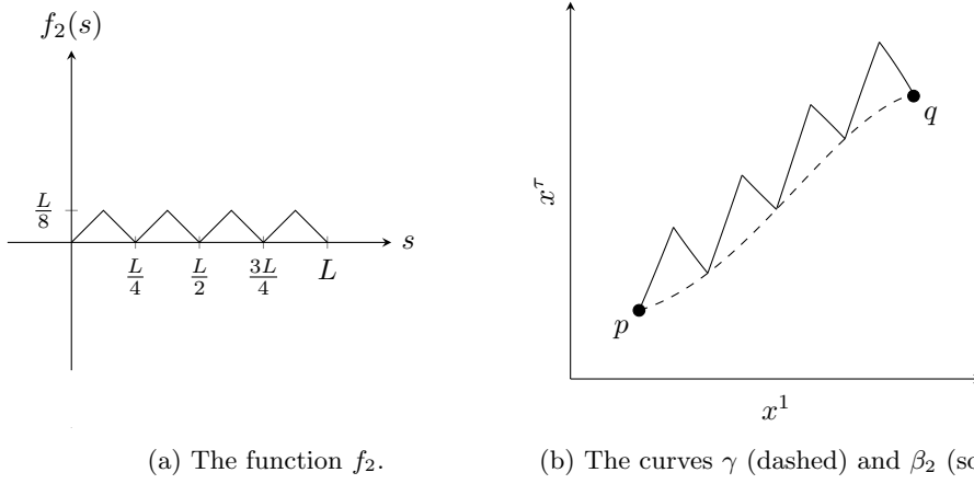
Figure 6.1: Illustration of the proof of Lemma 6.15.
