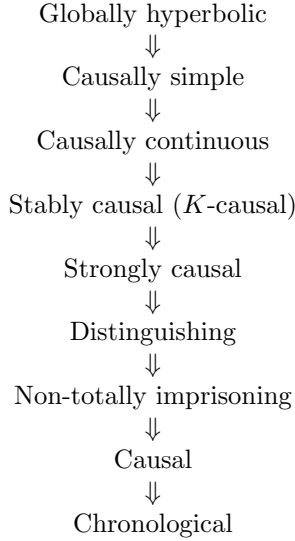
Figure 1.4: The causal ladder.
