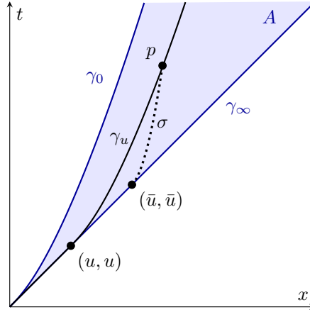
Figure 3.1: The causal bubble A as in Proposition 3.1.
