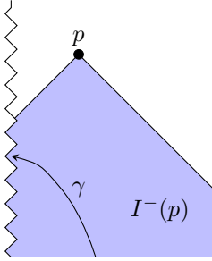
Figure 1.6: A locally naked singularity, represented by the zig-zag line.
