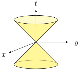
Figure 1.1: The lightcone.
