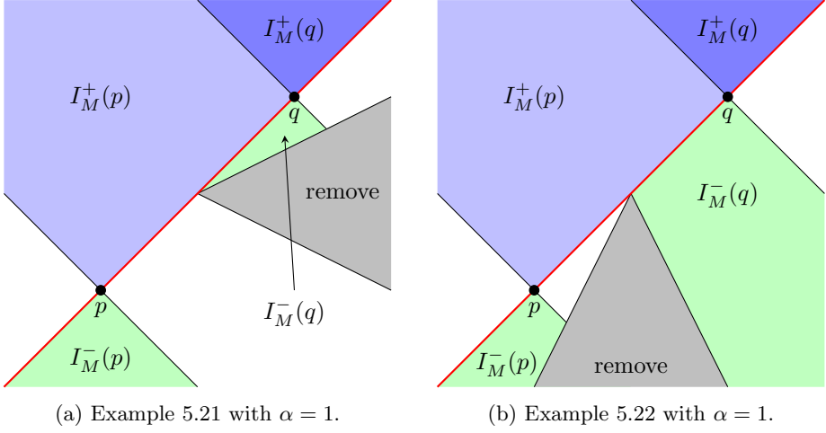
Figure 5.5: A pair of points p, q for which reflectivity is violated.
