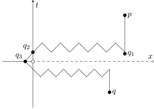
Figure 6.2: A piecewise causal curve that approximates the distance between the points p and q in Example 6.32, giving the upper bound (6.41).
