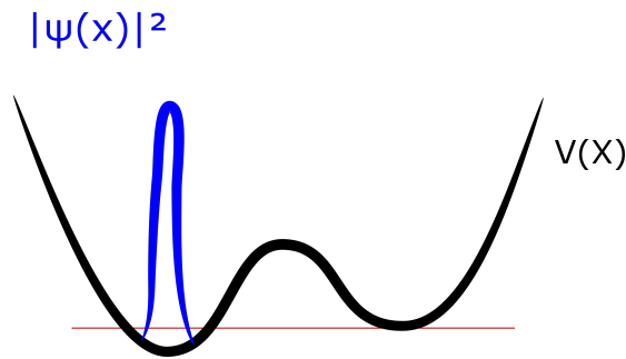
Figure 3.5: An almost classical object in the ground state. It is localized in the left well, since it fits almost completely inside the part of the left well that is completely below the lowest point of the right well (red line).
