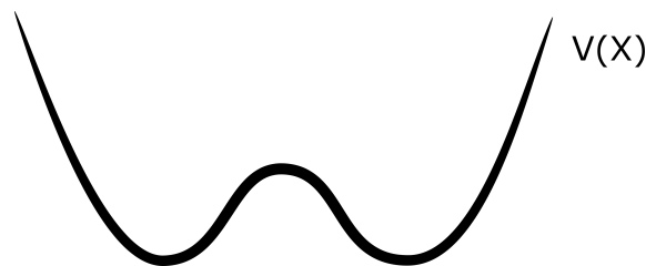
Figure 3.1: A symmetrical double well potential.
