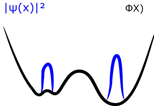
Figure 5.5: The gravitational potential after some part of the wave function has tunneled to the lower well.
