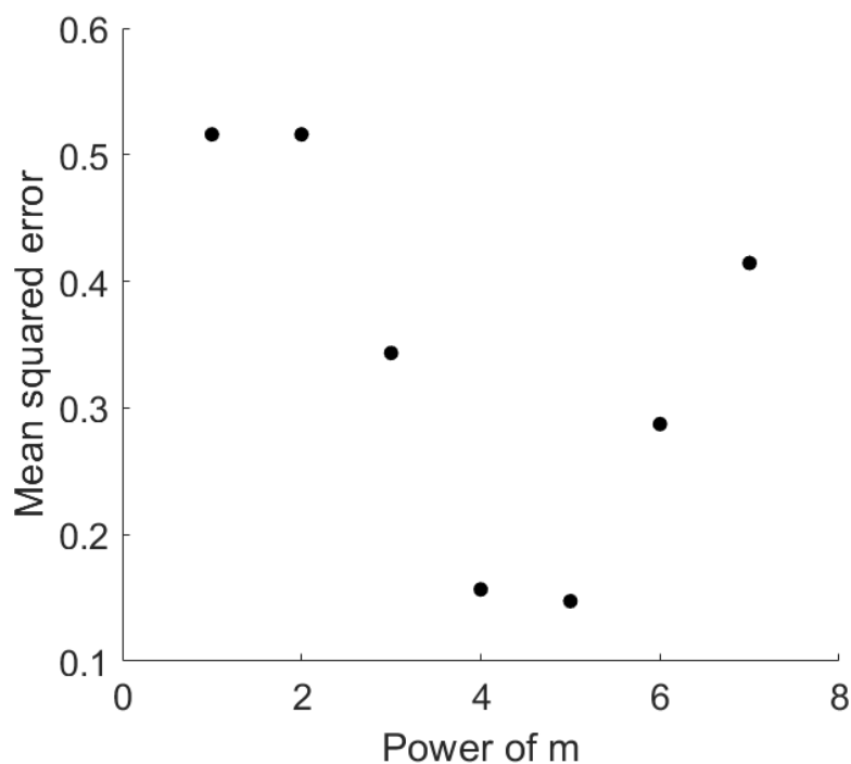
Figure 5.13: The minimal mean squared error of the derived probabilities compared to the Born probabilities for each possible power of m in equation (5.4). The mean squared error for a power 5 is 0.1474 which is slightly lower than for a power 4, which has 0.1567.
