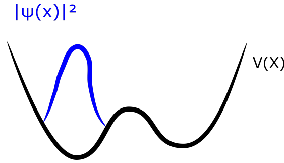
Figure 3.3: A quantum object in the left well.
