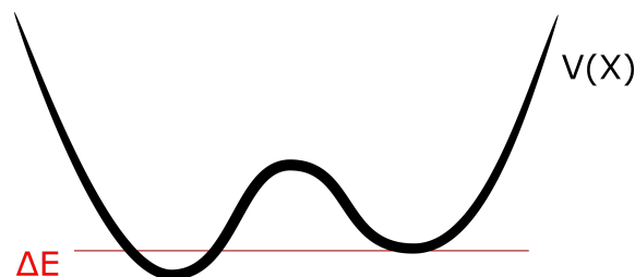
Figure 3.2: A biased double well potential with energy difference \Delta E .
