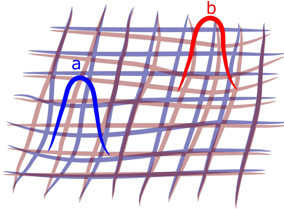
Figure 4.2: The system in a superposition \frac{1}{\sqrt{2}}(|a\rangle + |b\rangle) , with its induced space-time.
