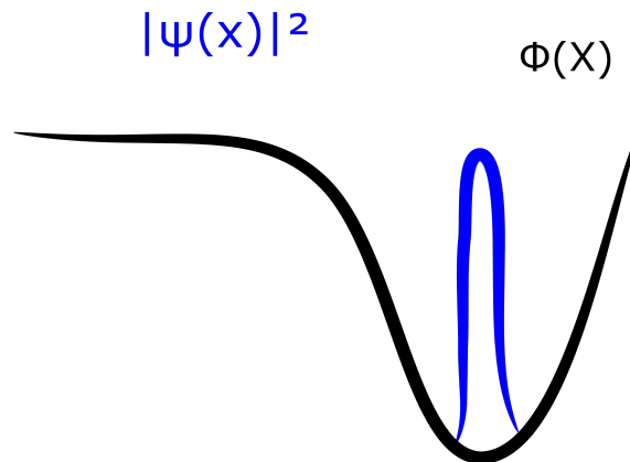
Figure 5.6: The gravitational potential after the wave function has collapsed to a single well.
