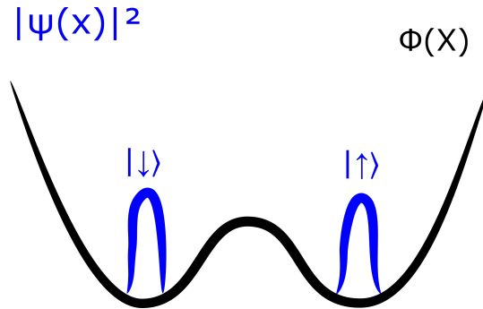
Figure 5.3: The gravitational potential corresponding to the superposition state.
