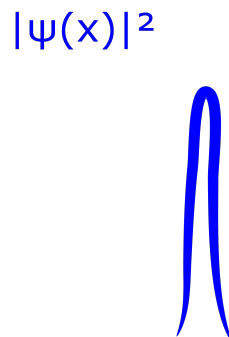
Figure 5.1: The device in its initial state.
