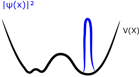
Figure 3.10: A small perturbation in the left well. The global minimum of the potential is now in the right well, so the entire wave function localizes there.
