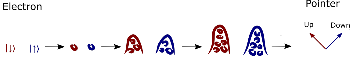
Figure 5.10: The superposition of the electron couples gradually to increasingly larger objects, until finally it couples to the entire pointer.
