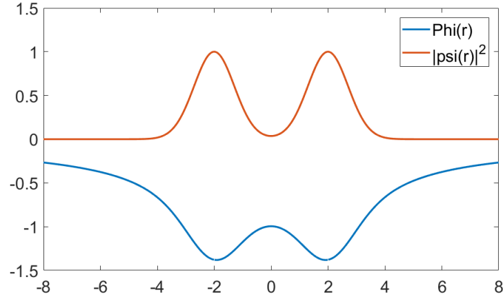
Figure 4.4: A plot of a wave function in a superposition of two Gaussians with \sigma = G = m = 1 , centered around -2 and 2. The corresponding gravitational potential \Phi(r) is also plotted.
