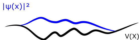
Figure 3.6: The ground state of a quantum system in some arbitrary potential. It has peaks at multiple minima.
