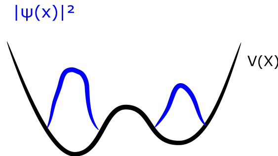
Figure 3.4: A quantum object in the ground state. It occupies both wells.
