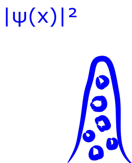
Figure 5.8: The initial state of a measurement apparatus consisting of many particles.
