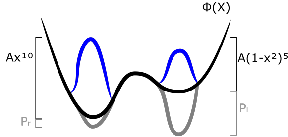
Figure 5.11: The double well with perturbations in each of the wells. Here the wave function would tunnel to the left.
