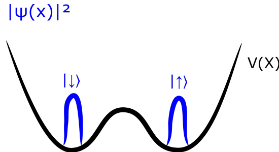
Figure 3.9: The measurement device coupled to an electron in superposition. The left peak is coupled to spin down, while the right peak is coupled to spin up.
