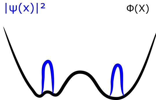
Figure 5.4: The gravitational potential plus some small perturbation.
