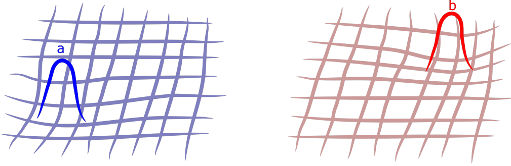
(a) The system localized around a and its induced space-time G_a . (b) The system localized around b and its induced space-time G_b .
