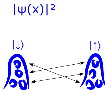
Figure 5.7: A wave function consisting of many particles. The particles have been drawn as circles. There is self-interaction, since different particles in the different parts of the wave function interact with each other.
