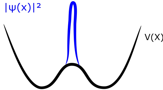
Figure 3.8: The initial state of a measurement apparatus.
