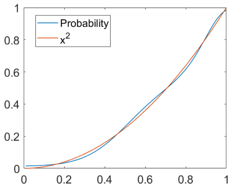
Figure 5.12: The derived probabilities (blue line) plotted against the Born probabilities (red line). The proportionality constant c is taken to be 0.4644, since this gives the best match.
