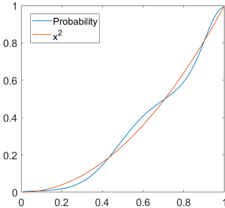
Figure 5.14: The derived probabilities for V(0) proportional to m^6 (blue line) plotted against the Born probabilities (red line). The proportionality constant c is taken to be 0.394, since this gives the best match.
