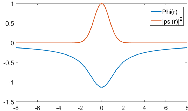
Figure 4.3: A plot of a Gaussian wave function density |\psi(r)|^2 with \sigma = G = m = 1 , centered around 0. The corresponding gravitational potential V(r) is also plotted.
