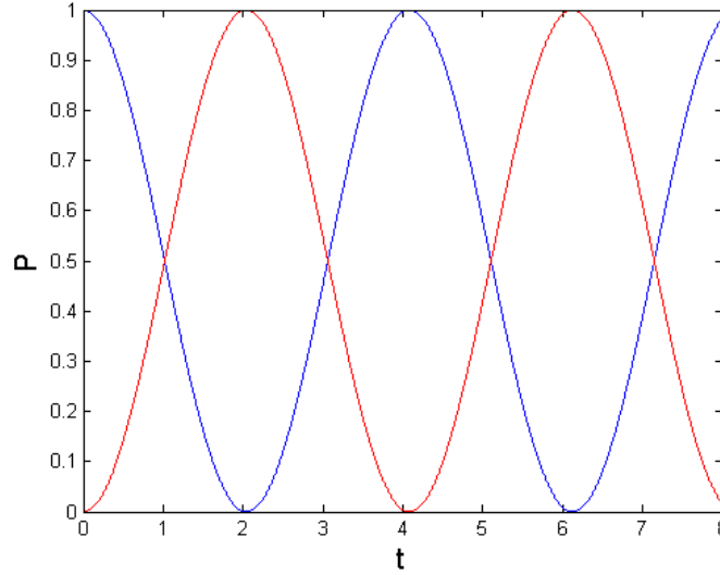
Figure 4.1: Time evolution of the probabilities P_L(t) and P_R(t) for the two-level system without perturbation and initial state \psi_L .
