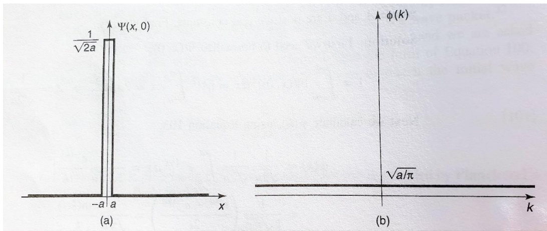
Figure 2: In these graphs we see an example of the wave function of a quantum particle in position and momentum space. The left graph shows the wave function for the position. It peaks in a very small interval while being zero elsewhere, so we can predict quite precisely where the particle will turn up upon measurement. The right graph shows the wave function for the momentum. Since this curve is equal in height across the entire interval, we cannot make a precise prediction of the momentum at all. The curve is much lower because the total area beneath it must sum up to 100%
