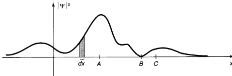
Figure 1: An example of the absolute value of the wave function squared, which according to Born is to be interpreted as the probability of finding the particle at a certain location upon measurement. The grey area tells you the probability of finding the particle in the interval dx . We require that the total area beneath the curve is equal to 100% since we are certain to find the particle somewhere. This is called 'normalization'. Given the height of the curve, it is likely that the particle will appear near A, less likely so near C and very unlikely near B (Griffiths, 2014, p. 3).
