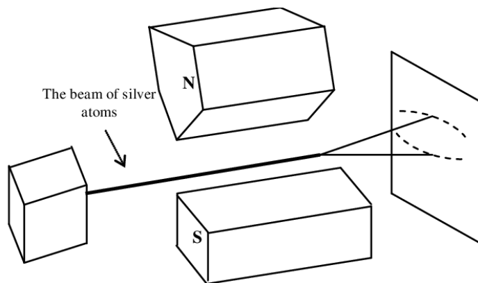
Figure 3: A simplified portrayal of the Stern-Gerlach experiment. Silver atoms in the beam are, when passing through the magnetic field, either deflected upward a certain amount or downward by the same amount. This is the influence of spin (Erkoç, 2009).
