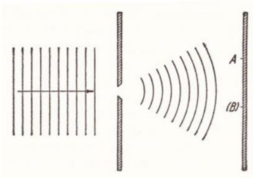
Figure 7: A visualization of Einstein's single-slit thought experiment. A photon passes through the slit in a screen and diffracts. The second screen is a photographic plate that detects the photons at a specific point (Kumar, 2008, p. 264).
