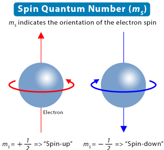
Figure 4: A pictorial representation of the classical analogue of spin. In this analogy, the electron is a small sphere spinning about an axis (here the z-axis), with the counterclockwise spinning being called 'spin-up' (+1/2) and the clockwise spinning being called 'spin down' (-1/2) (Spin Quantum Number, 2022).
