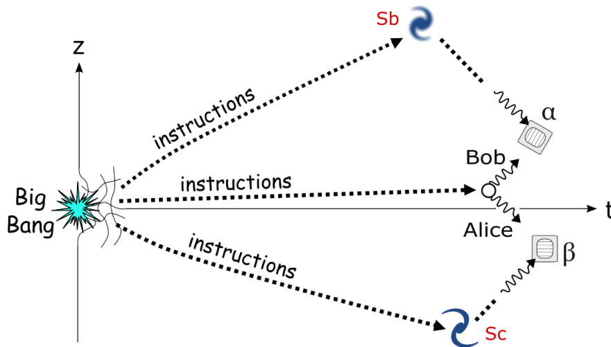
Figure 12: A visualization of correlations present in the universe from the big bang onwards (Dalton, 2021).
