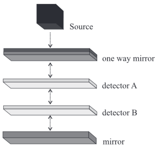
Figure 14: The experimental setup with which a subset of superdeterministic models could be tested, as contrived by Hossenfelder. The source emits a particle with a small probability of passing the mirror. The particle is then likely to travel up and down many times, being subjected to measurements of two non-commuting variables by detector A and B. Since according to quantum mechanics the measurement of one should destroy information of the other, this allows measurements on the particle to be made in rapid succession while the particle is effectively returned to its initial state each time (Hossenfelder S. , 2011, p. 7).
