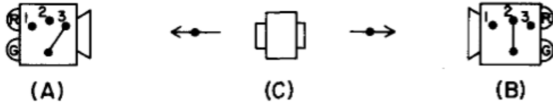
Figure 9: Mermin's realization of Bohm's EPR-setup. Two detectors A and B measure the spin of two entangled particles emitted from a source C. All parts are unconnected (Mermin, 1981, p. 400).
