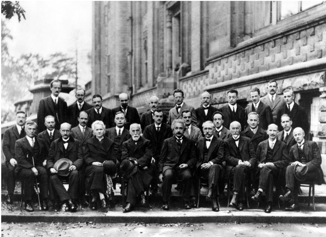
Figure 6: Attendants of the 1927 Solvay conference on Electrons and Photons. Bohr can be found at the right end of the middle row, while Einstein is seated in the middle of the third row (Solvay conference 1927 (group photograph), 2020).
