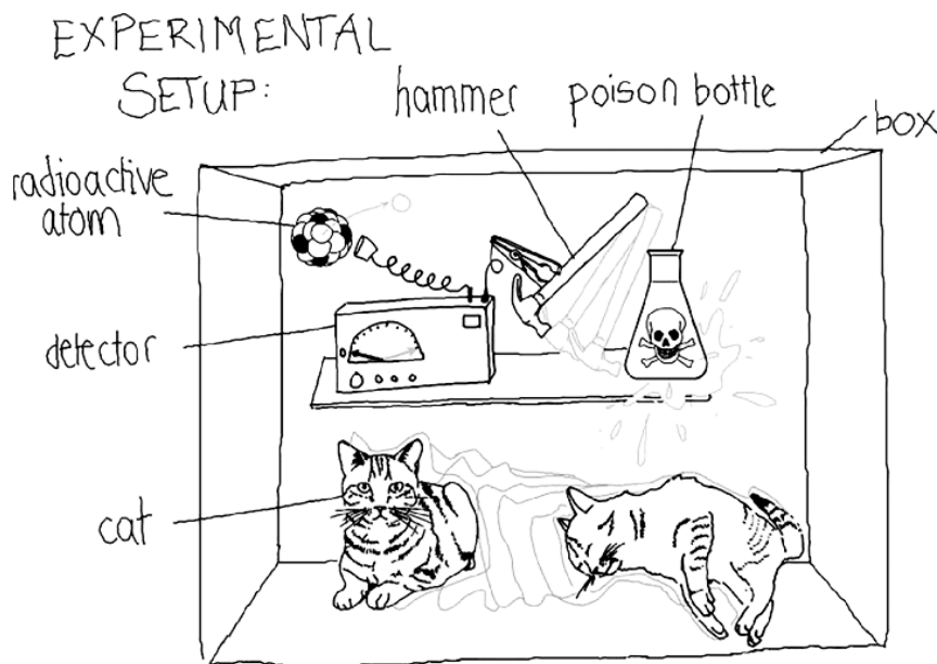
Figure 8: The experimental setup of the Schrödinger's cat thought experiment (Hartjes, 2016). The fate of the cat is decided by the probabilistic process of a radioactive atom decaying or not.
