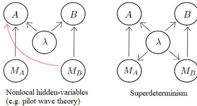
Figure 13: A nonlocal hidden-variable theory compared to a superdeterministic hidden-variable theory. In the nonlocal case, atoms have a real state characterized by \lambda , but changing the measurement setting at detector B causes a faster-than-light signal changing the spin of atom A later measured at detector A (again in a Bohm-Mermin type setup). In the superdeterministic case, no such signal is present, but rather, pre-existing correlations represented by \lambda account for observations that appear to imply signaling (Sen & Valentini, Superdeterministic hidden-variables models I: nonequilibrium and signalling, 2020, p. 10).
