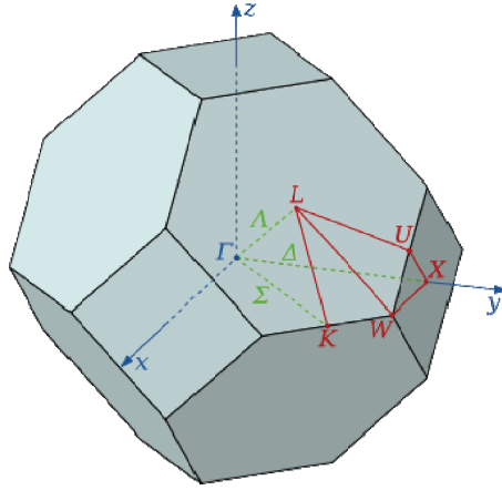
Figure 31: A Wigner-Seitz (or Voronoi) cell for the cubic lattice in \mathbb{R}^3 . Figure from Wikipedia.
