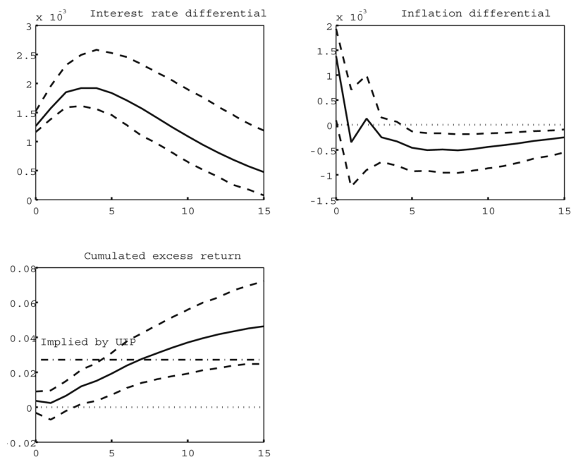
Fig. 6. Impulse response functions from VAR(3) for shock to interest rate differential with 90% confidence intervals.
