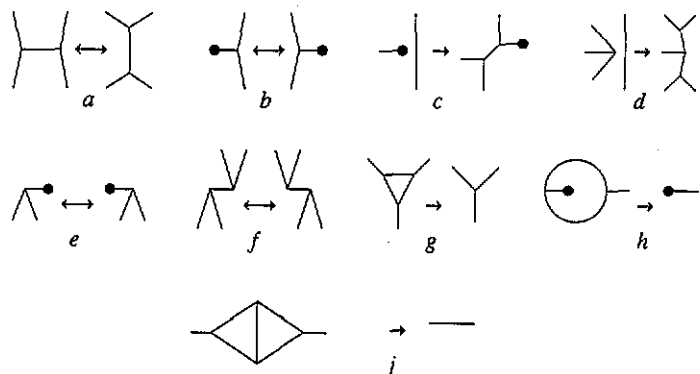
Figure 1. Schematic diagrams of the nine different possible transitions.
