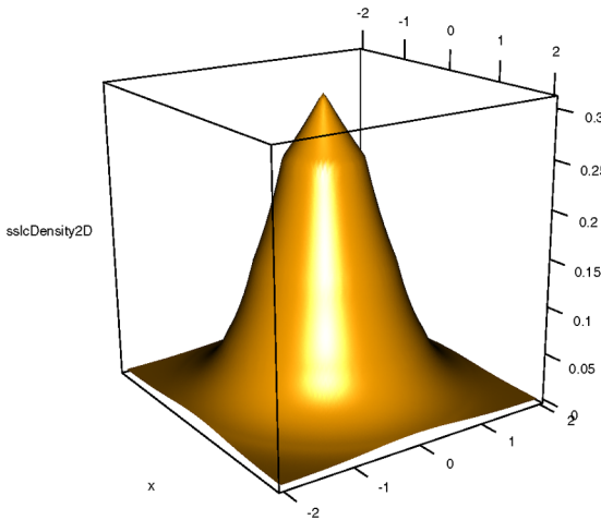
FIG. 8. A comparison of the spherically-symmetric log-concave MLE \hat{f}_n^{\text{SS}} (left) and the estimator \tilde{f}_n defined in (8.2) (right) based on a sample of size n = 1000 from a standard bivariate normal distribution.
