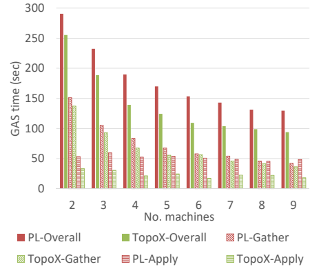
Figure 12: Comparison of overall, Gather, Apply times between TopoX and PowerLyra (PL).
