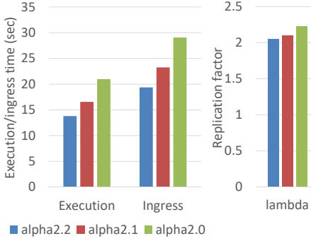
Figure 14: TopoX Performance on various \alpha (2.0, 2.1 and 2.2).
