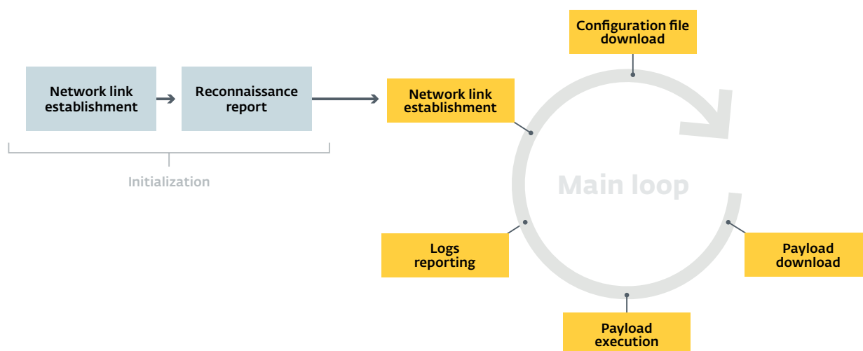
Figure 16. Seduploader's payload workflow
