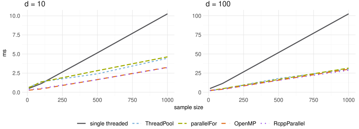
Figure 4: Time required for computing the kernel density estimate in parallel for d variables.
