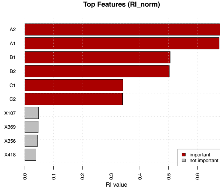
Figure 4: Top features selected by MCFS-ID.
