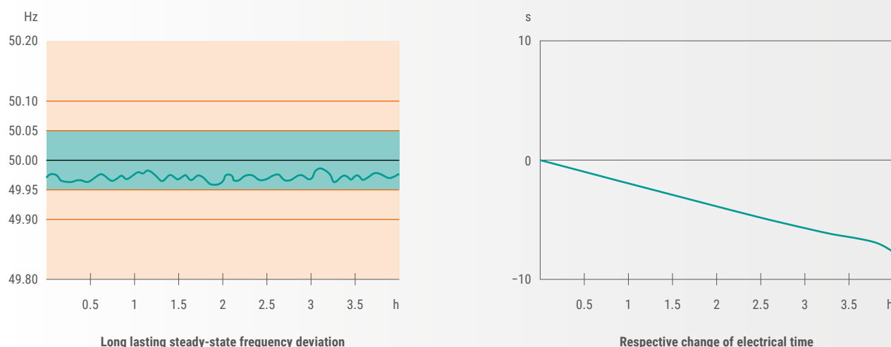
Figure 1: Relationship between frequency deviation and electrical time
