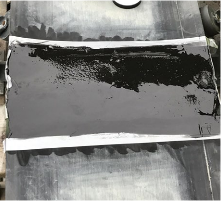
After Metal Clips Splice Repair
