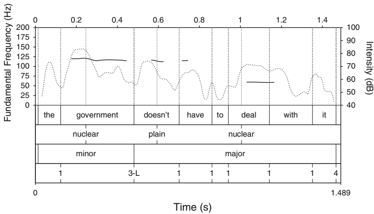
Fig. 3 Example Praat textgrid and acoustic display of the prosody annotation (part of the utterance from Fig. 4). The fundamental frequency track (solid line) and intensity curve (dotted line) are shown, along with the phonetic transcript, the accent annotation ( accent type marked ), the phrase annotation ( type marked ), and break annotation (break index and phrase tone marked)
