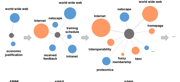
Figure 7: Illustration of the dynamic graphs that capture interactions between search engine and its co-occurrence concepts. The orange circles denote transferred concepts while the blue denotes non-transferred ones; the circle size represents the node degree.
