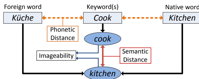
Figure 2. Illustration of the mnemonic keyword learning strategy. Effective keywords are phonetically similar to the foreign word, correspond to highly imageable concepts, and are semantically close to the concept. Concepts in dark blue circles, word forms in light blue boxes.
