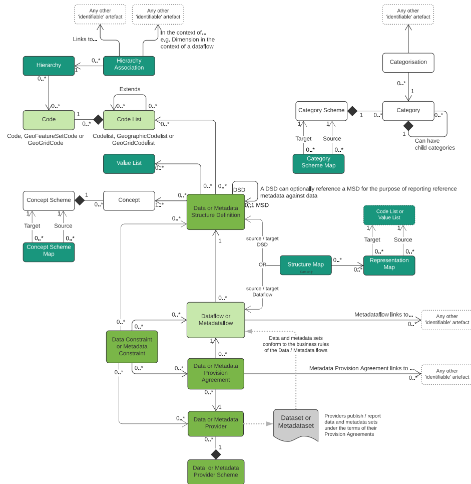
70 Figure 1 Version 3.0 simplified Information Model UML class diagram with 'heat map' illustrating the areas with most change
