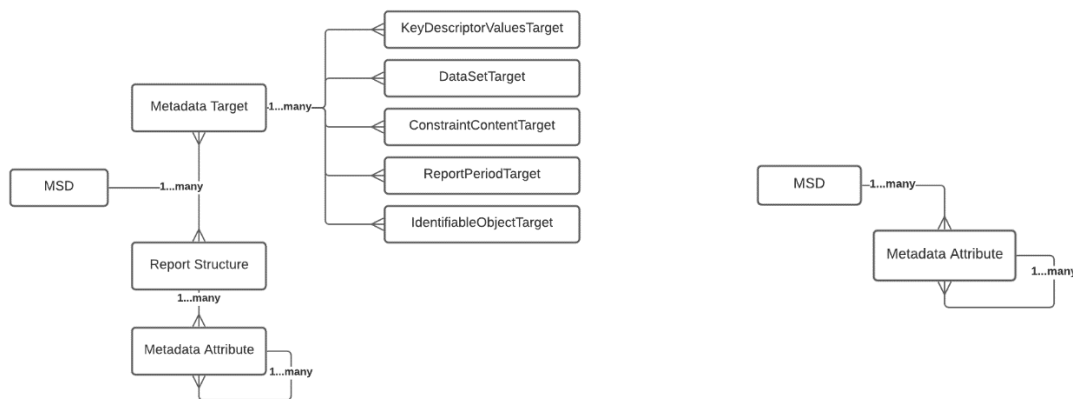
Figure 2 version 2.1 Metadata Structure Definition (MSD)
