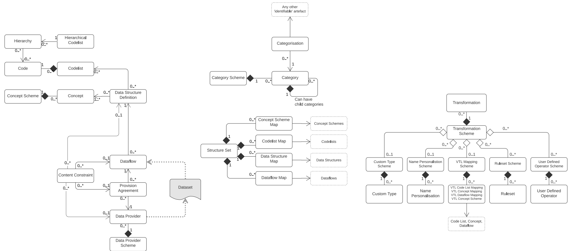
Figure 4 Version 2.1 simplified Information Model UML class diagram
