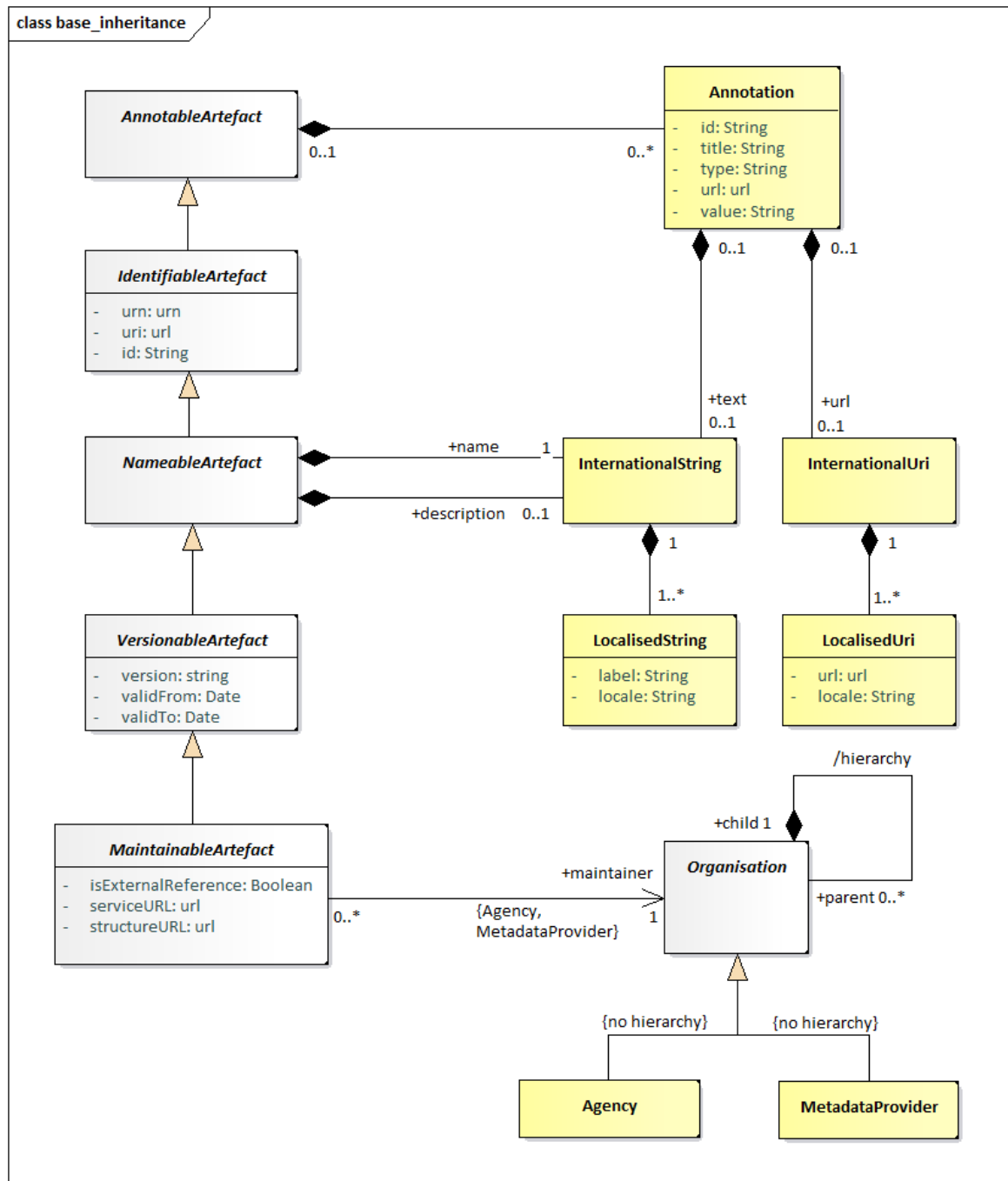
343 344 Figure 5: Class diagram of fundamental artefacts in the SDMX-IM
