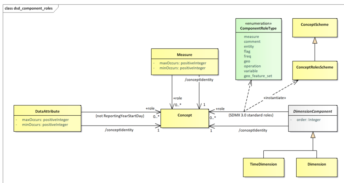
Figure 19: Information Model Extract for Concept Role
