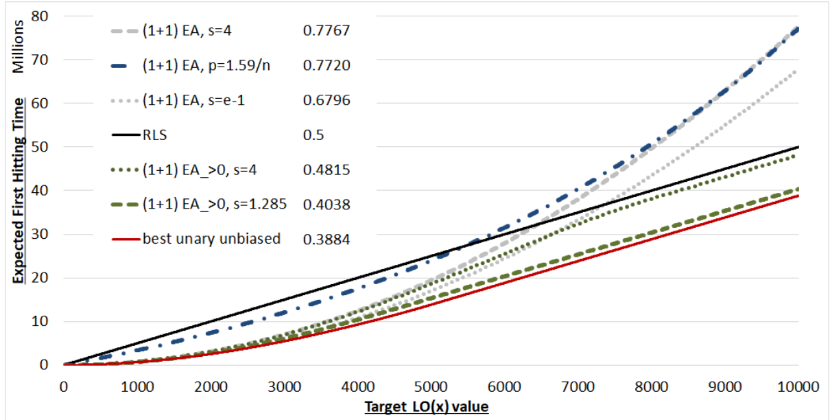
Figure 3: Expected fixed target running times for LEADINGONES in dimension n = 10000 . The curve of (1+1) \text{ EA}_{>0,\text{opt}} is indistinguishable from that of the (1+1) \text{ EA}_{>0} with success ratio s = 1.285 and the curve of the (1+1) \text{ EA}_{\text{opt}} indistinguishable from that of the (1+1) \text{ EA} with success ratio s = e - 1 . The values shown in the legend are the expected optimization times, normalized by 1/n^2 .
