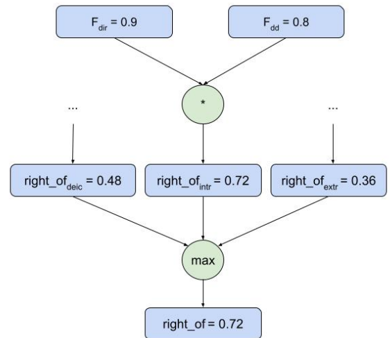
Figure 3: An example of an explanation procedure.
